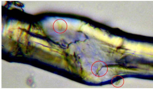
Fig. 7. (Color online) Microscope image of a single linen fiber colored after ArF laser irradiation. The mechanical damage in the central part allows observation of small broken pieces of colored primary cell wall (see inside circles) on a colorless inner part of the fiber. The average diameter of the fiber is 20 \mu\text{m} .
