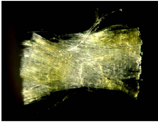
Fig. 4. (Color online) Photomicrograph of a warp thread of flax irradiated with ArF laser at a total laser fluence F_T = 26.4 \text{ J/cm}^2 . The thread was crushed with forceps to separate the fibers and highlight their yellow color. At the center of the thread, there is a uncolored zone due to a weft thread that shadowed the laser radiation [36].
