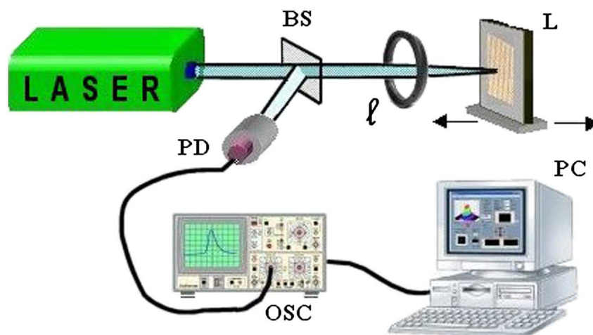
Fig. 2. (Color online) Setup of excimer laser irradiations of linens. The laser pulses are focused by the lens \ell on the linen fabric L. The laser fluence/intensity on the linen is varied by moving L along the optical axis of the lens. Part of the laser pulse is reflected by the beam splitter BS and monitored by the photodiode PD and the oscilloscope OS connected to a personal computer PC, which processes the data, taking into account the shot-to-shot energy fluctuations. The distance between the XeCl and the ArF excimer lasers and the lens is about 1 m and 25 cm, respectively.
