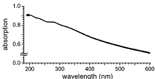
Fig. 11. Plot of the absolute value of the absorbance of the linen versus the wavelength, according to our experimental values inserted in Eq. (3). The thickness of the plot gives the error associated to the measurement.
