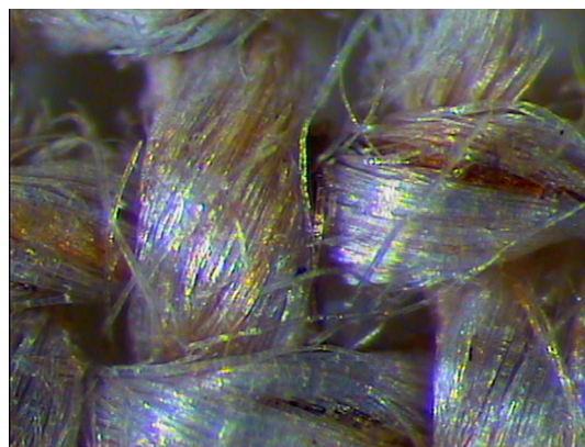
Fig. 16. (Color online) Photomicrograph of linen threads after ArF laser irradiation. Single colored fibers are visible next to uncolored fibers, like in the Shroud image.
