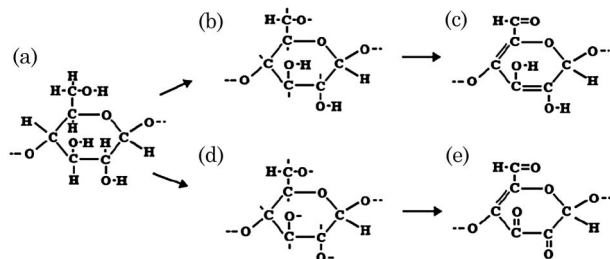
Fig. 14. (a) Main molecular structure common to both cellulose and hemicellulose. There are two possible transitions (a) \rightarrow (b) \rightarrow (c) and (a) \rightarrow (d) \rightarrow (e) that generate chromophores after oxidation and dehydration. The C=C and C=O double bonds in (c) and (e) act as chromophores and are responsible for the yellow color of the fibers of image on the Shroud of Turin.
