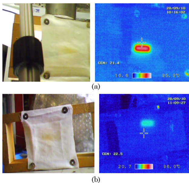
Fig. 13. (Color online) (a) (Left) Photo of the linen during XeCl laser irradiation. (Right) Same picture seen in infrared light. The color scale at the bottom shows that the warmest region of the linen (in the middle of the laser spot) reaches 33°C, while the nonirradiated area is at the room temperature of 20°C. (b) (Left) Photo of the linen during ArF laser irradiation. (Right) Same frame seen in infrared light. The color scale reveals that the warmest area of the irradiated linen is at 25°C, while the nonirradiated area is at the room temperature of 21°C.
