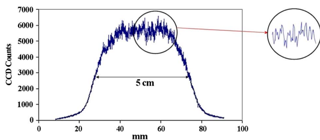
Fig. 15. (Color online) One-dimensional intensity/fluence profile of our laser beam measured by a CCD camera Andor Model DV-430UV, with a 22 \mu\text{m} single-pixel resolution. The inset shows an enlargement of the high-frequency spatial fluctuations. Note that the contribution of CCD noise to the spatial fluctuations on the plateau is negligible, of about 4 \times 10^{-3} .
