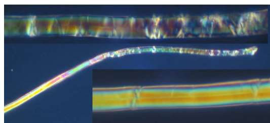
Fig. 12. (Color online) Petrographic microscope observation of a linen fiber. In the middle there is a partly colored fiber of linen in oil 1.515 between crossed polarizers. The left part of the fiber is the nonirradiated region, which is enlarged in the inset below. On the right there is the region irradiated by XeCl laser, enlarged in the inset above. From [32].
