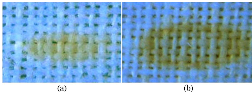
Fig. 9. (Color online) Blue fluorescence induced by UV lamp on linen after irradiation with ArF laser. (a) In the working point of the third row of Table 1. The irradiated area shows a reduced fluorescence. (b) By using a laser beam having a “holed” spatial profile of the intensity. In this case the fluorescence reduction is not uniform over the whole laser spot.
