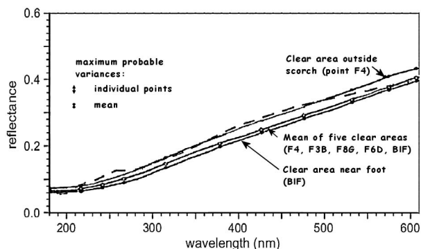
Fig. 10. The solid curves show the absolute reflectance of the linen of the Shroud in areas of no image as a function of the wavelength [3]. The dashed curve shows the absolute hemispherical reflectance of the linen used in our experiments [35].
